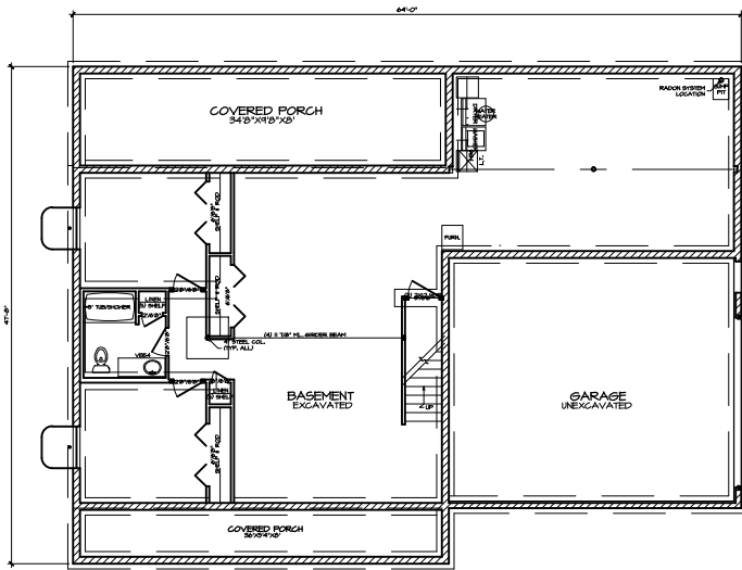
FOUNDATION PLAN A-3
