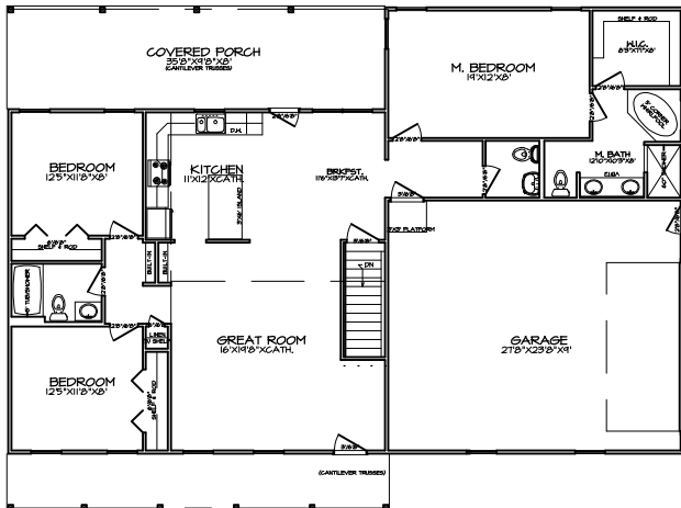
FIRST FLOOR PLAN A-4
